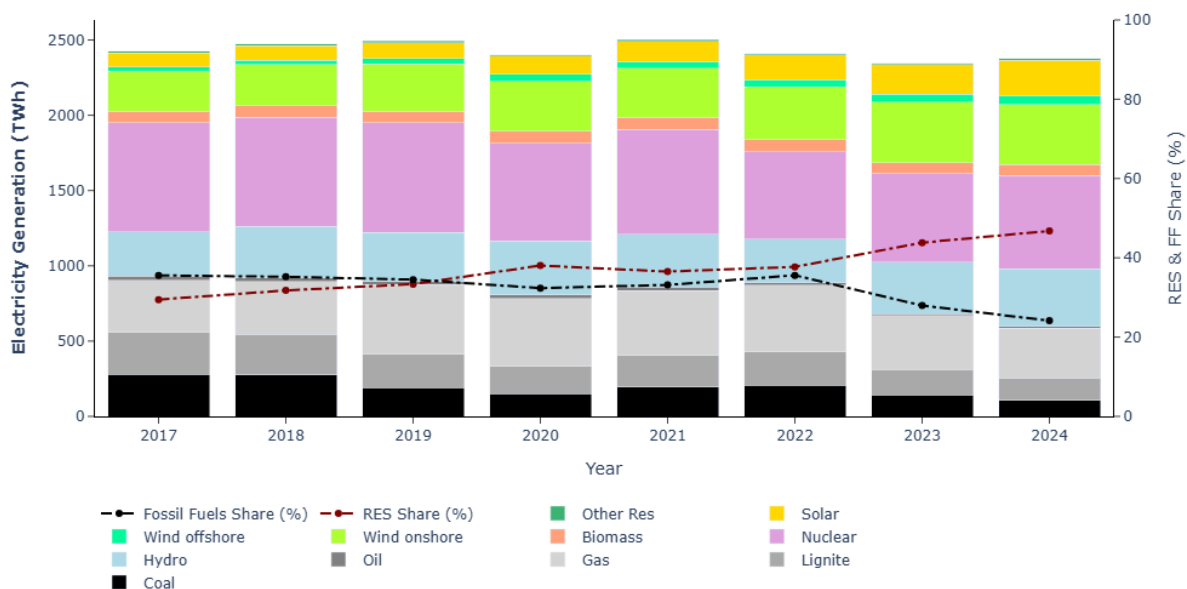
Figure 19 – Yearly electricity generation mix in the EU
